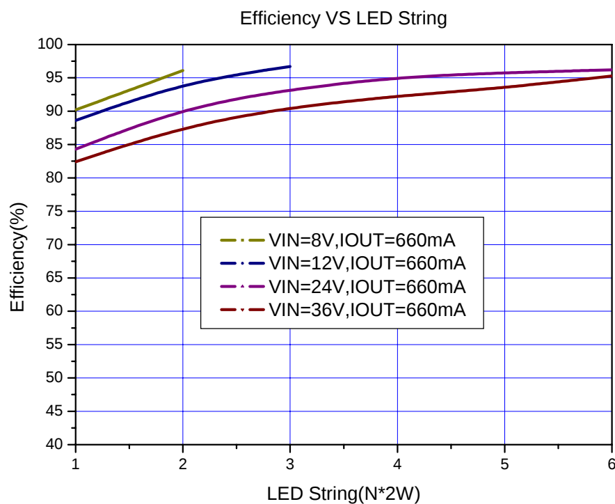
Figure19. CM5201 System Efficiency Curve (VIN=8V~40V,IOUT=660mA)
