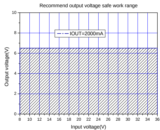
Figure15.Max output voltage(IOUT=2000mA)
