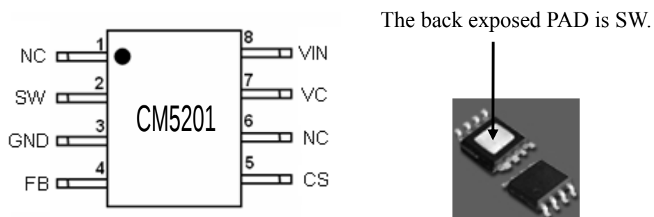
Figure2. Pin Configuration of CM5201 (Top View)
