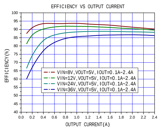
Figure8. Efficiency Curve
