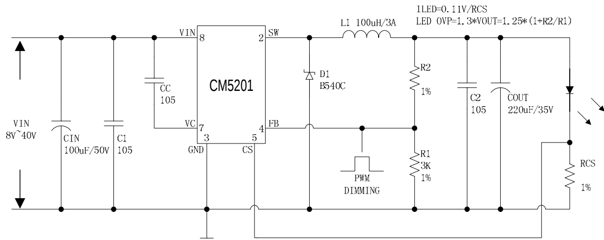
Figure22. CM5201 System Parameters Test Circuit
