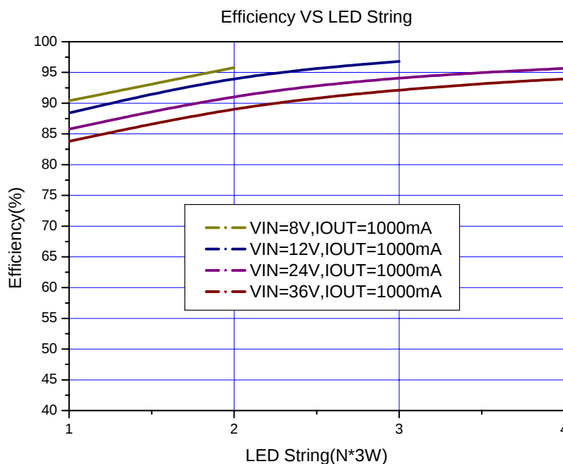
Figure21. CM5201 System Efficiency Curve (VIN=8V~40V,IOUT=1000mA)
