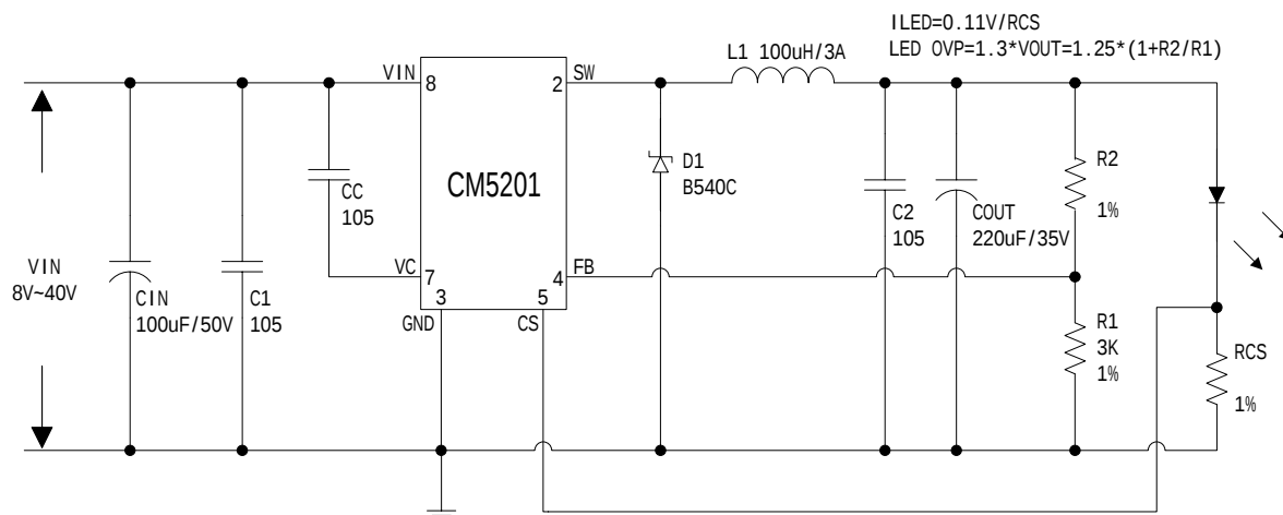
Figure5. CM5201 Typical Application Circuit(LED Constant Current Driver)
