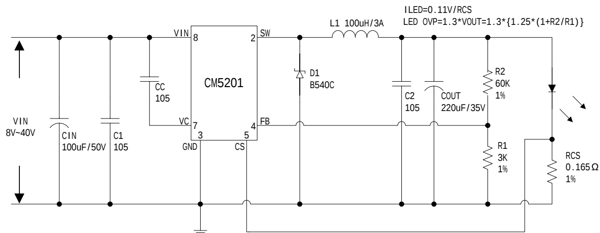
Figure18. CM5201 System Parameters Test Circuit (VIN=8V~40V,IOUT=660mA)
