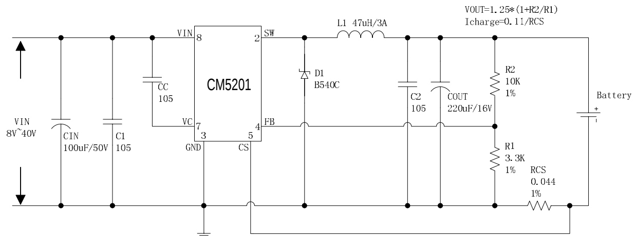
Figure6. CM5201 System Parameters TestCircuit (VIN=8V~40V, VOUT=5V/0.1A~2.5A)
