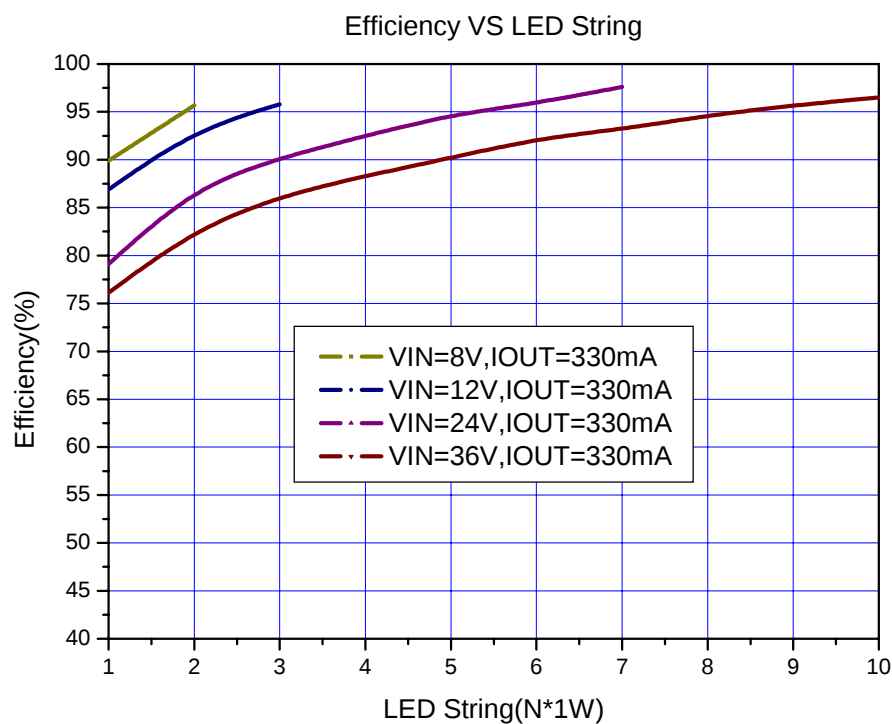
Figure17. CM5201 System Efficiency Curve (VIN=8V~40V,IOUT=330mA)
