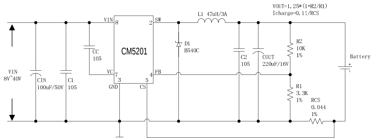
Figure4. CM5201 Typical Application Circuit (Li Battery Charger)
