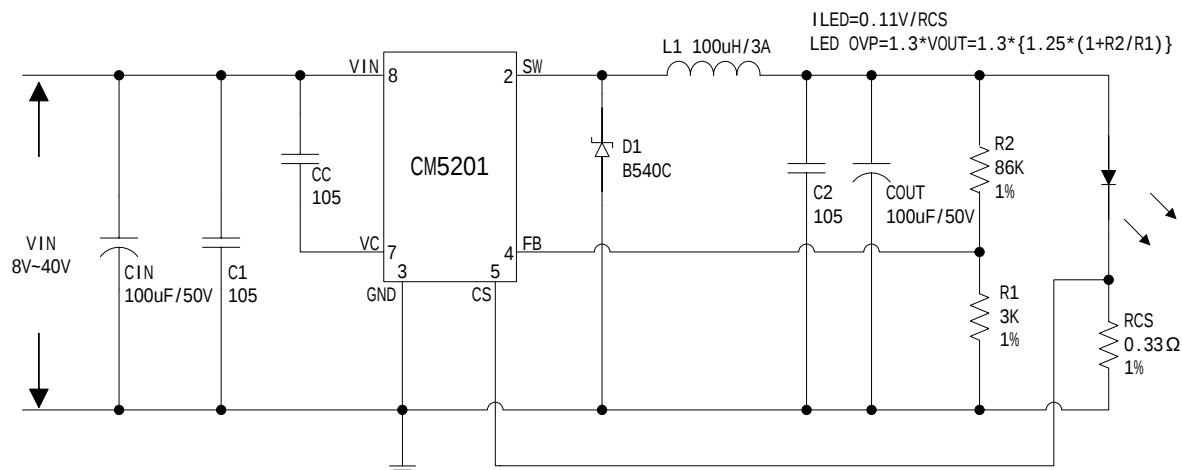
Figure16. CM5201 System Parameters Test Circuit (VIN=8V~40V,IOUT=330mA)
