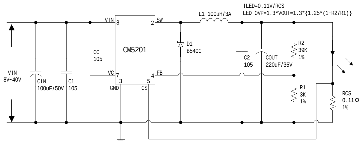
Test Circuit (VIN=8V~40V,IOUT=1000mA)
