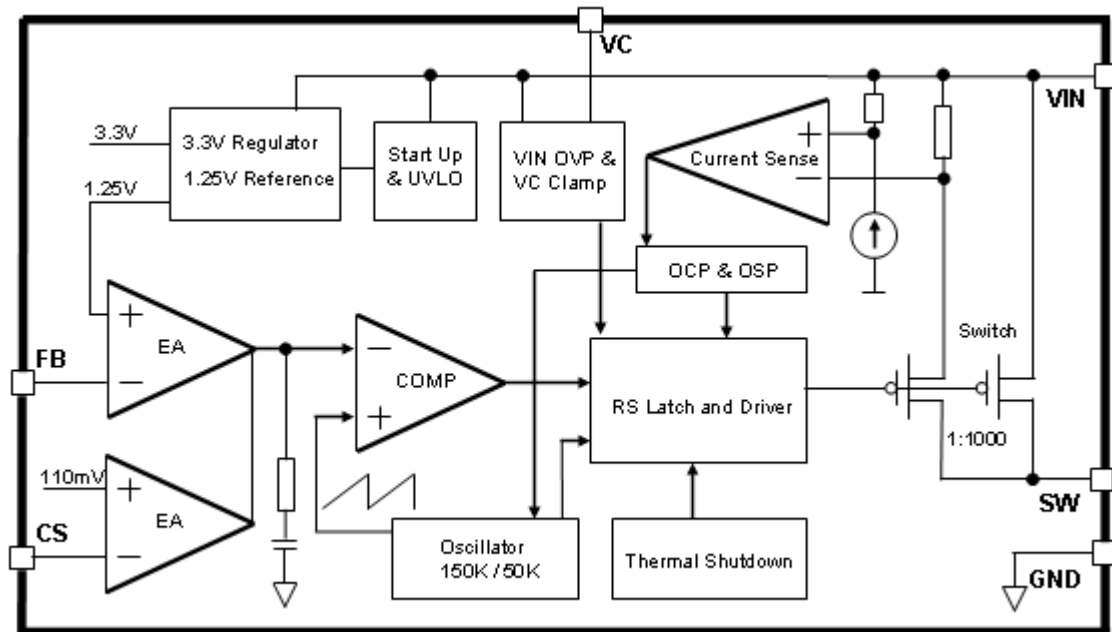
Figure3. Function Block Diagram of CM5201
