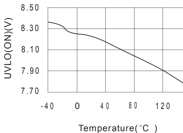
UVLO(ON)(V) vs Temperature(°C )
