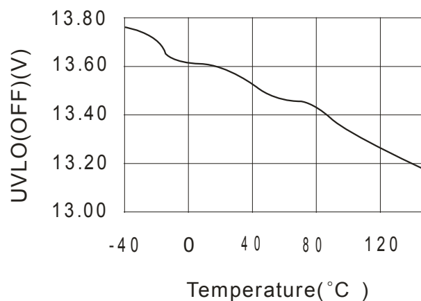
UVLO(OFF)(V) vs Temperature(°C )
