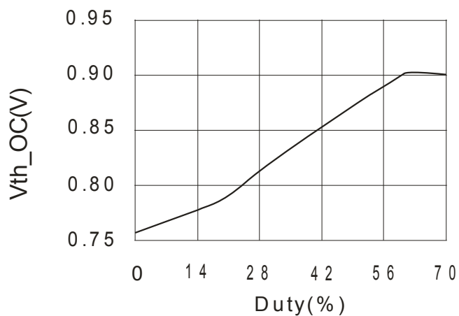
Vth_OC(V) vs duty(%)
