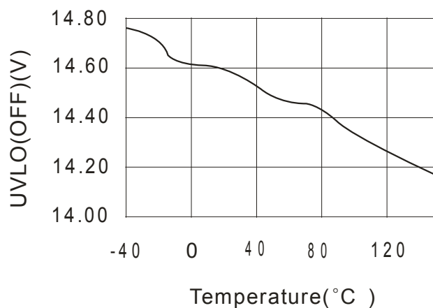
UVLO(OFF)(V) vs Temperature(°C )
